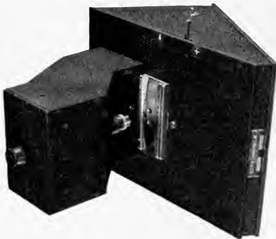
FIG. 2. View showing lever (4, Fig. 1), film-gate, and eyepiece.
